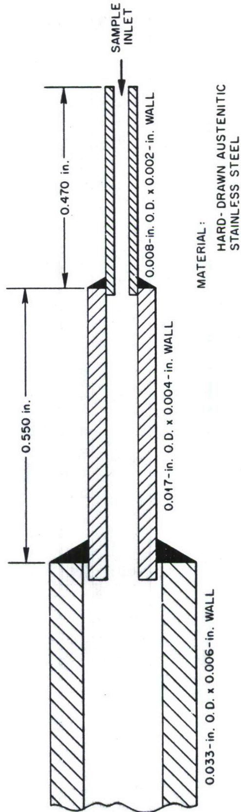
Fig. 18. Sample Probe Detail.
