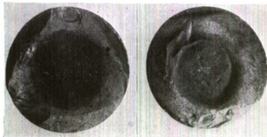
FIG. 7. Fracture surfaces of silicon nitride gudgeon pin.
