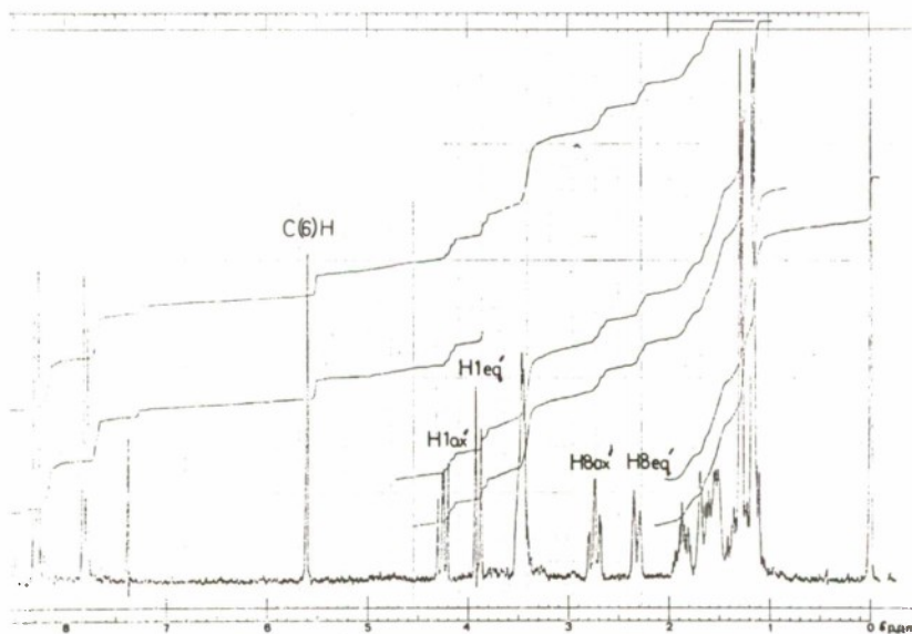
FIG. 6. 220 MHz n.m.r. spectrum of 6- p -nitrophenyl-2,3-dimethyl-perhydropyrido [1,2- c ] [1,6,3] dioxazocine.
