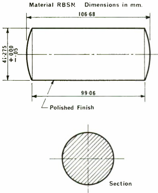
FIG. 4. Gudgeon pin design in RBSN.
