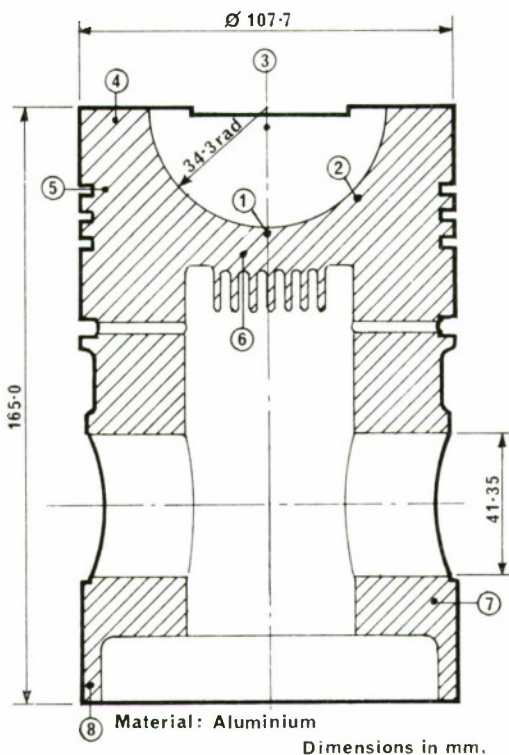
FIG. 1. Section through original piston.
