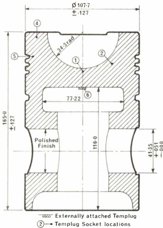
FIG. 2. Section through final piston design.
