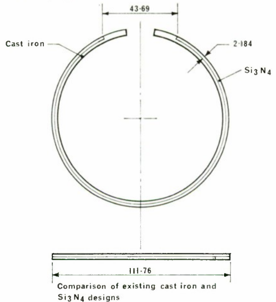
FIG. 3. Piston rings. Comparison of existing cast iron and silicon nitride designs.
