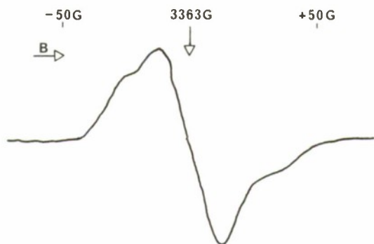
FIG. 1. Typical Spectrum from DGEBA cured with DDM.
