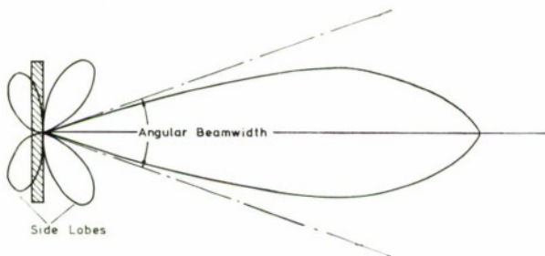
FIG. 3. Directional response (in polar form) of a disc transducer.
