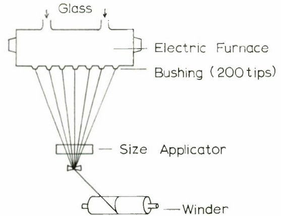
FIG. 1. A typical fibre forming arrangement.
