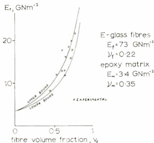
FIG. 4. Transverse Young's modulus for glass fibre reinforced epoxy.
