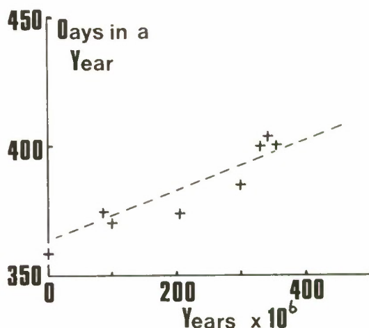
FIG. 1. Coral fossil evidence of lengthening day.
