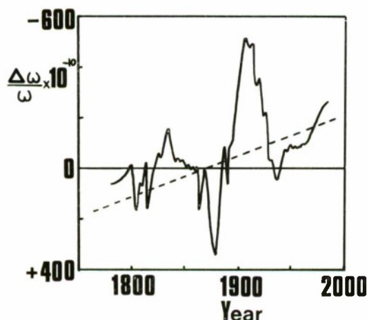
FIG. 3. Results of author's measurements of Moon's motion compared with Theory.
