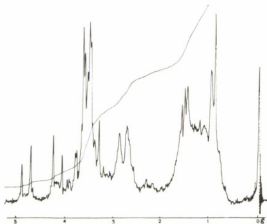
FIG. 11. 60 MHz n.m.r. spectrum in \text{CHCl}_3 of the mixed isomers of 9-ethyl-perhydropyrido [1,2- c ] [1,6,3] dioxazocine after the decomposition of one isomer. The peak at \delta 2.95 p.p.m. was removed by shaking the solution with deuterium oxide.
