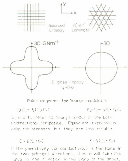
FIG. 8. Directional properties of various fibre configurations.
