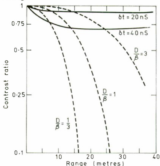
FIG. 6. Fall-off of target contrast with range in water with \alpha = 0.2\text{m}^{-1} . The contrast is improved using the geometrical isolation method by
