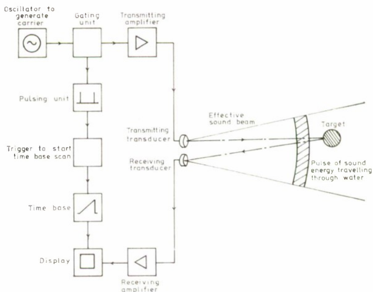
FIG. 2. Schematic arrangement of a typical pulsed sonar system.
