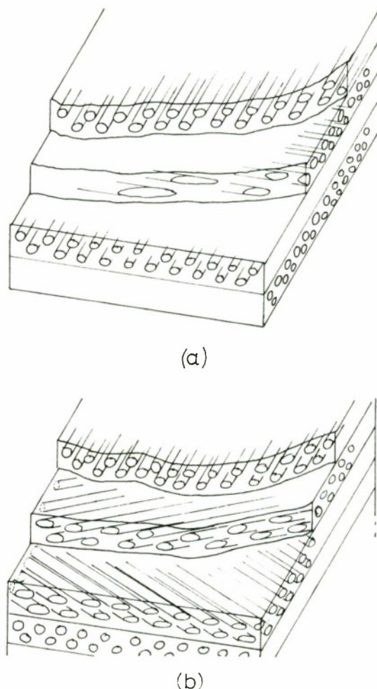
FIG. 7. Schematic diagrams showing the stacking sequence in (a) a simple crossply. (b) a 0^\circ, \pm 60^\circ laminate.
