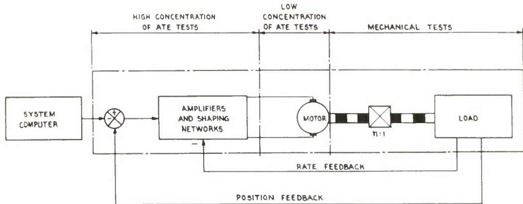
FIG. 3. Block schematic of large electro-mechanical system.
