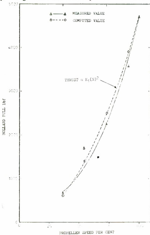
FIG. 9. Bollard pull tests — Bollard pull against propeller speed.
