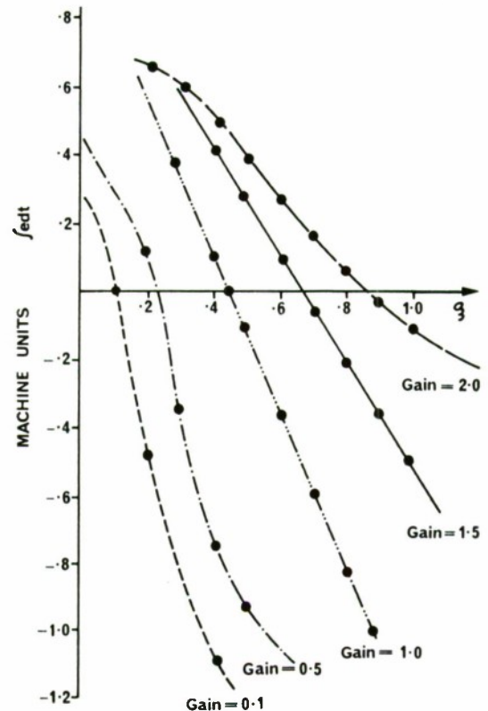
FIG. 3. Graph of f_{edt} against \xi for various values of gain.
