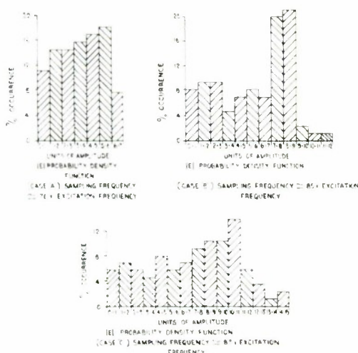
FIG. 8. Automation of 'finger printing': error distributions resulting from low frequency sine wave test.
