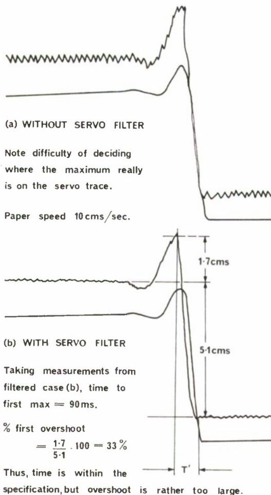
FIG. 2. Analogue Model trace and servo system trace \times 100 .
