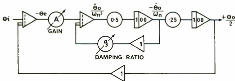
FIG. 1. Block diagram of model reference system.
