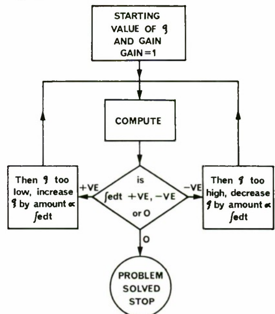
FIG. 4. Flow diagram of iteration sequence for \xi adjustment.
