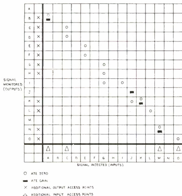
FIG. 6. Access point matrix for system tested by ATE.
