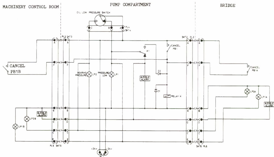
FIG. 8. Oil low level pressure alarm system for the auxiliary pumping unit.
