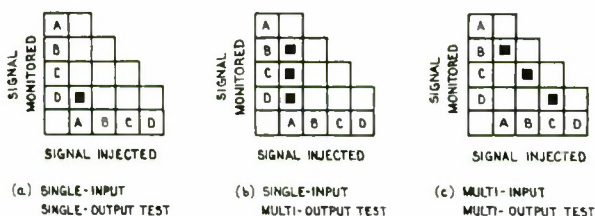
FIG. 1. Test point matrices.
