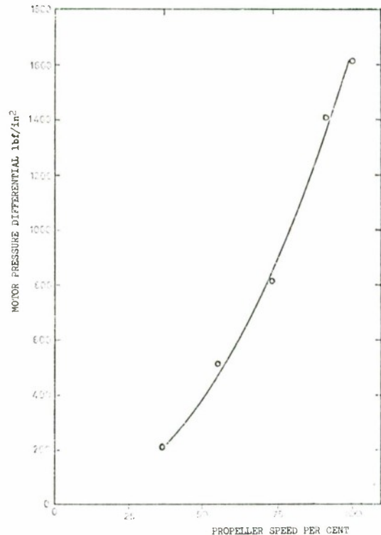
FIG. 10. Motor pressure differential against propeller speed.
