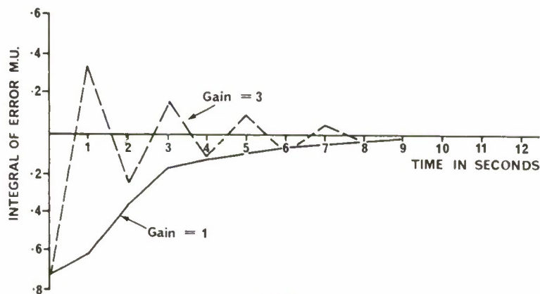
FIG. 5. Performance index for successive iterations for various values of gain.
