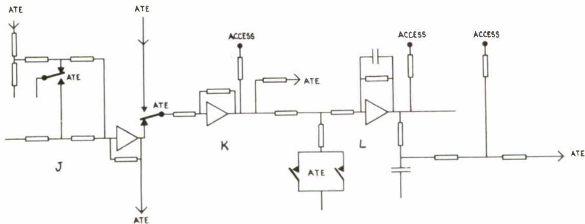
FIG. 7. ATE test circuit.
