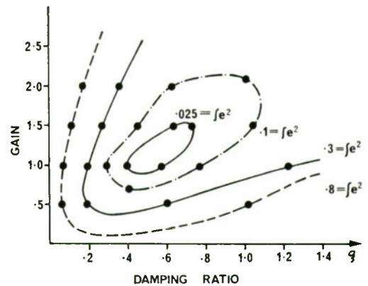
FIG. 7. Graph of gain against \xi showing contours of constant P.I.
