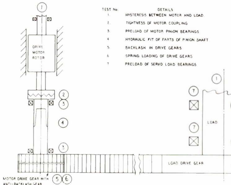
FIG. 4. Typical mechanical tests.
