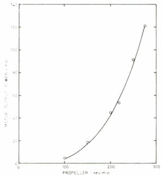
FIG. 11. Power output of motor for corresponding pressure differentials and propeller rev/min.
