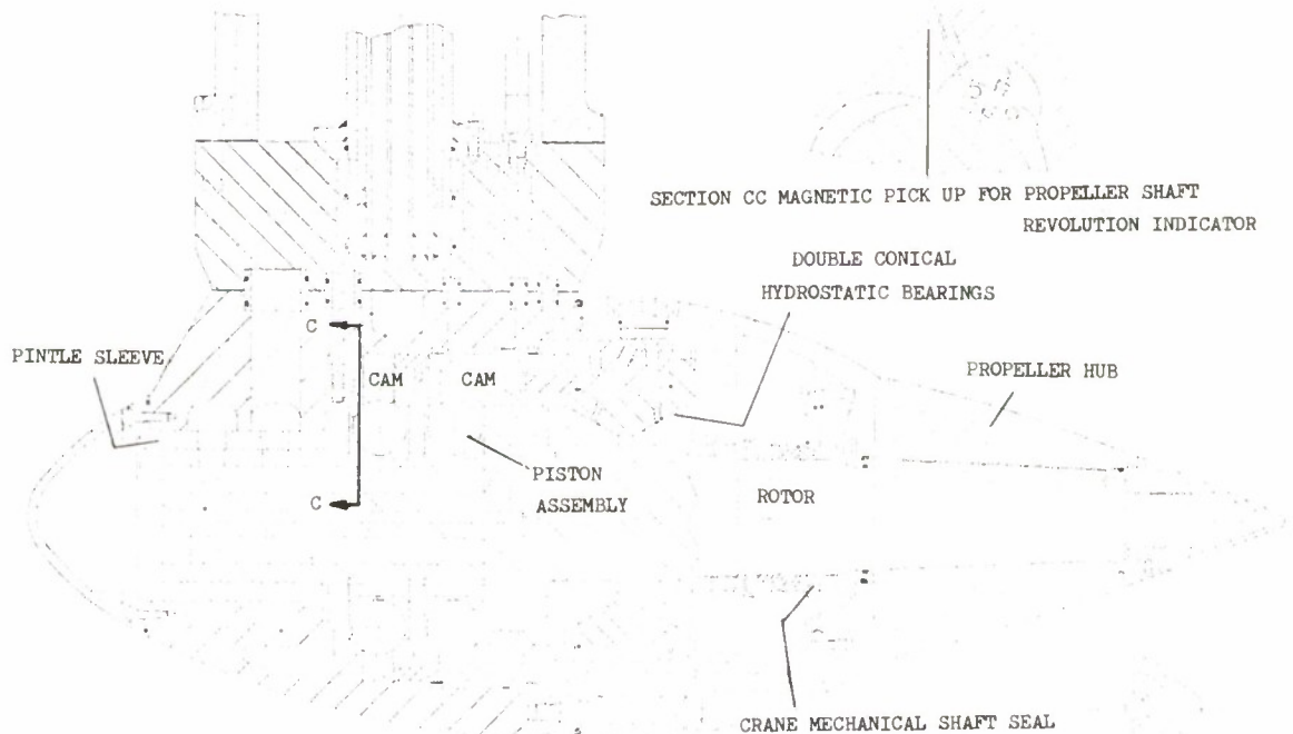
FIG. 6. Cross section through NEL 145 h.p. Podded ball motor showing manifold and lower end of concentric tube assembly.
