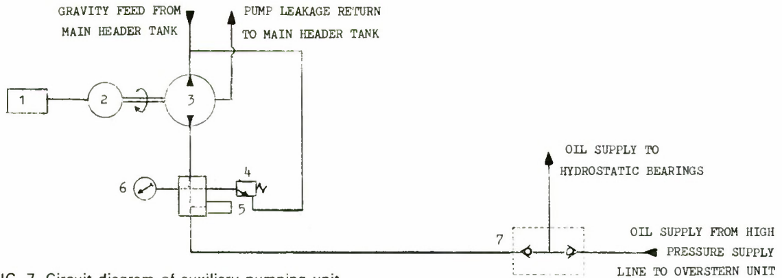
FIG. 7. Circuit diagram of auxiliary pumping unit.
