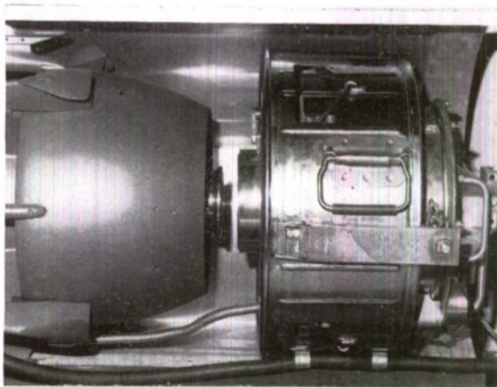
FIG. 5. This torpedo-mounted guidance wire dispenser was developed by NUSC to eliminate the problems associated with torpedo stowage, handling and guidance wire splicing onboard submarines.
