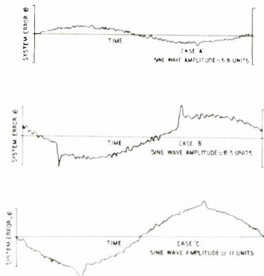
FIG. 5. Records of error channel dynamic tests.
