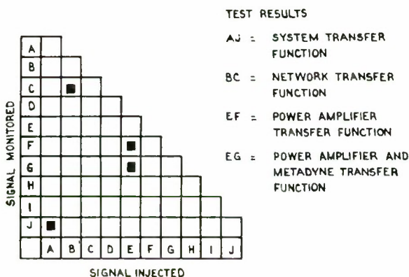
FIG. 2. Test point matrix for large electro-mechanical servo not designed for testing by ATE.
