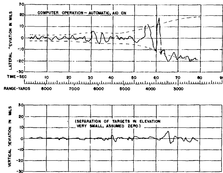
RADAR MK. 25 TRACKING 2 TBF'S SIDE BY SIDE AT 3000 FT. ALT.
