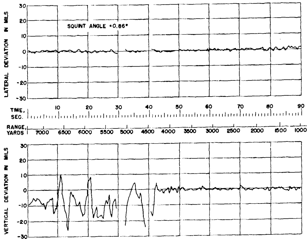
RADAR MK 7, MOD 1, TRACKING SNJ-3 AT 200 FT. ALTITUDE
