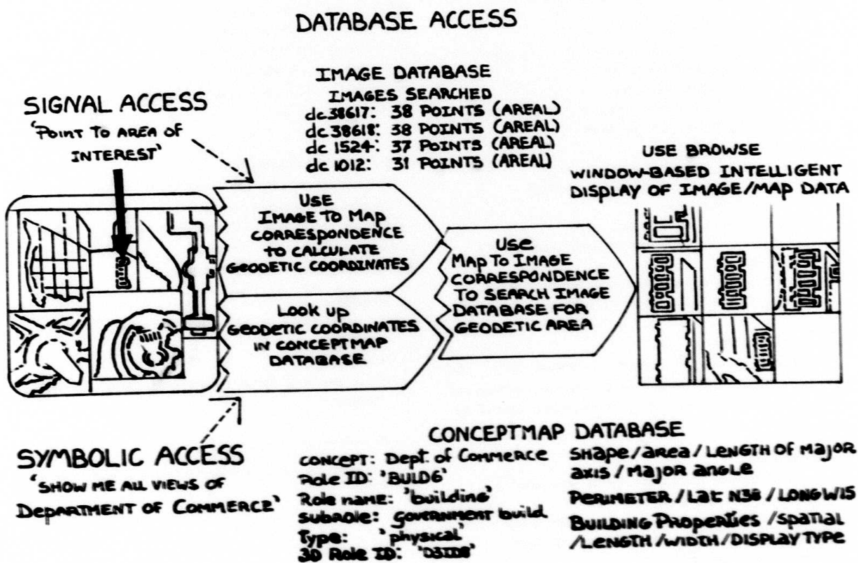
Figure 8: MAPS: Signal / Symbolic Database Access
