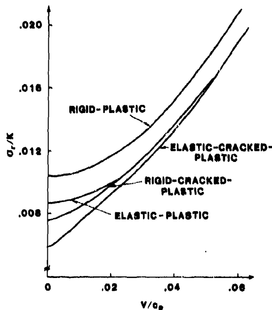
Fig. 1. Radial stress on the penetrator conical nose. V = V_z \tan \phi , c_p^2 = K/\rho_0 where V_z is axial penetrator velocity and \phi is the half apical nose angle.
