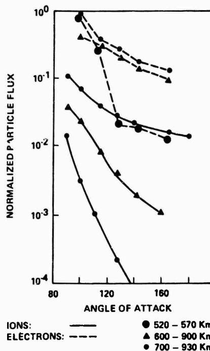
Figure 3. Variation of Normalized Ion and Electron Currents With Angle of Attack. Ions-solid line, electrons-dashed line for the altitude ranges: 520 to 570 km (●); 600 to 900 km (▲); 700 to 930 km (•), based on Explorer 31 and Atmosphere Explorer C measurements
