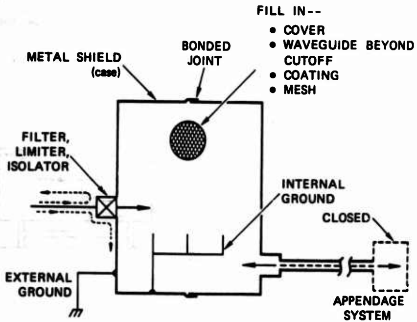
Fig. 5 - Elements of a typical closed electromagnetic barrier
