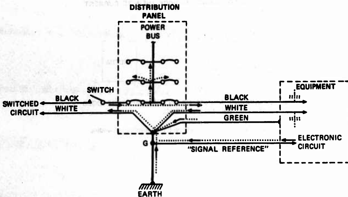
Fig. 10 - Interference distribution through an ill-conceived grounding system
