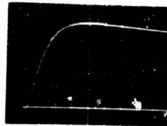
Fig. 3 - 2 x 50 \mu s Return Stroke into Aircraft Terminated with R_t = Z_o
