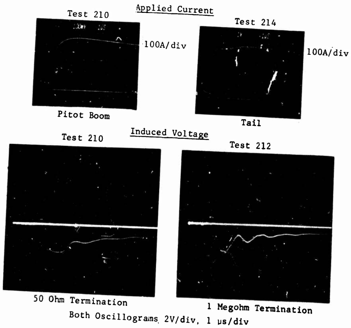
Fig. 15 - Induced Voltage Measurements 2 x 50 μs Wave
