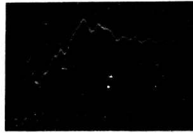
0.5A/div 100ns/div Return Current (return conductor)
