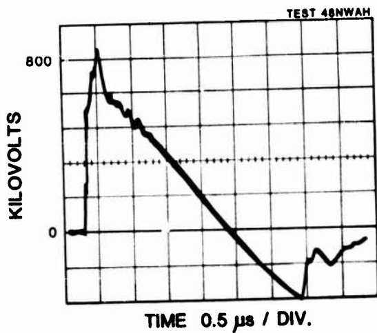
Fig. 12 - High-voltage pulse developed at nose of F/A-18 with 100-kA current pulse
