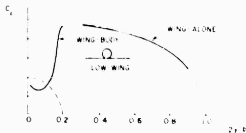
FIG. 4 SPANWISE LOAD DISTRIBUTIONS OF WING BODY CONFIGURATIONS
