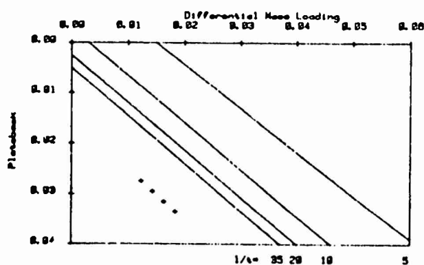
Figure 8 Differential mass loading as a function of plateback for the fundamental mode — Theory + Experiment ( t/t_0 = 14 )
