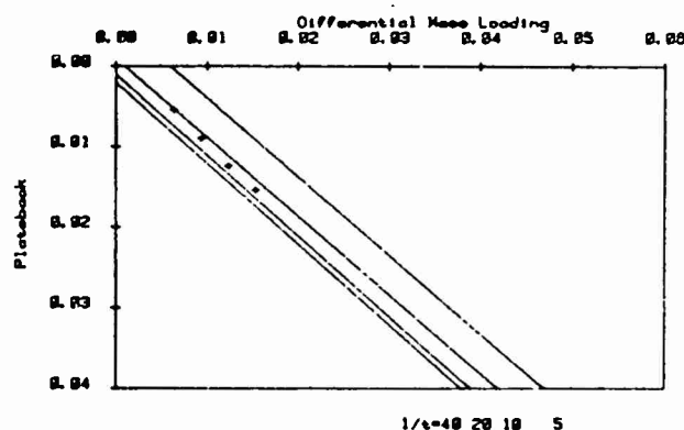
Figure 9 Differential mass loading as a function of plateback for the third overtone mode — Theory + Experiment ( t/t_0 = 14 )
