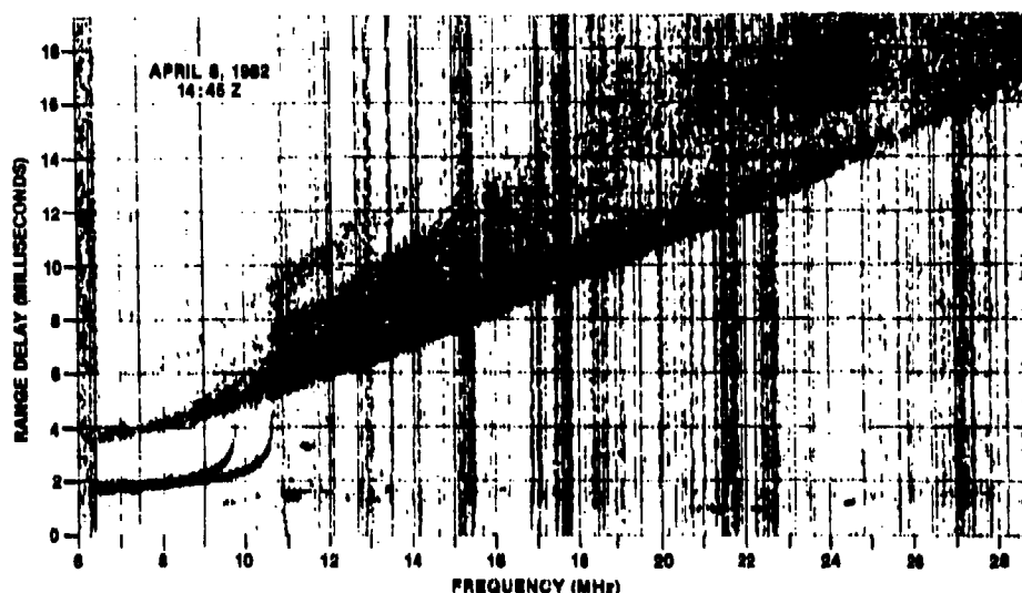
FIG. 5. Backscatter Ionogram
