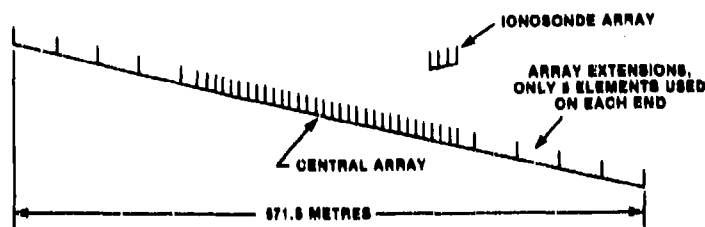
FIG. 3(c) Final Array Configuration Used for Sea-State Experiments
