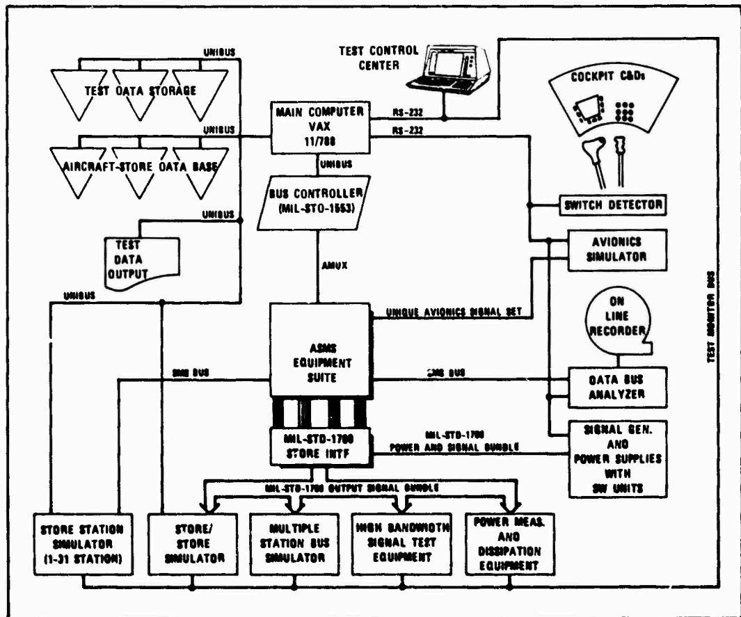
Figure 6. Advanced SMS laboratory for the study of interface and SMS requirements
