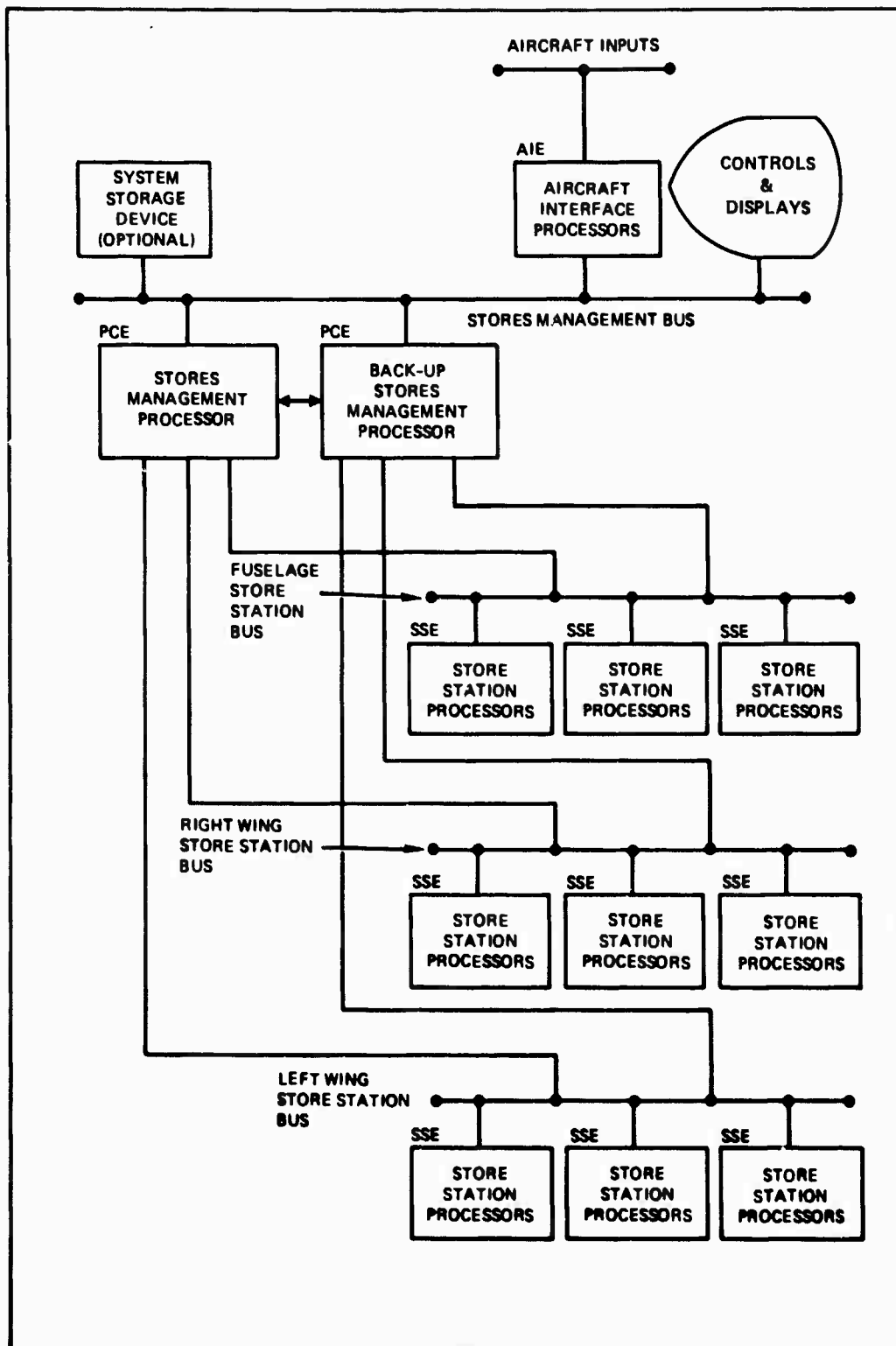
Figure 10. Contractor 8 SMS architecture with fiber optics data buses
