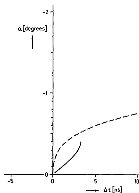
Figure 7. Path delay as function of \alpha , for B'_c = 1.0 * 10^{-7} \text{ [m}^{-1}] (solid line), and B''_c = 2.6 * 10^{-7} \text{ [m}^{-1}] (dotted line)
