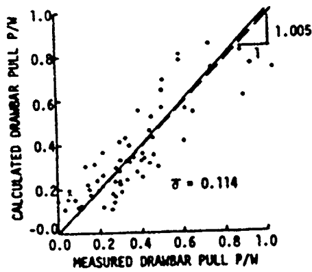
Figure 28. Predicted versus measured drawbar pull for clay
