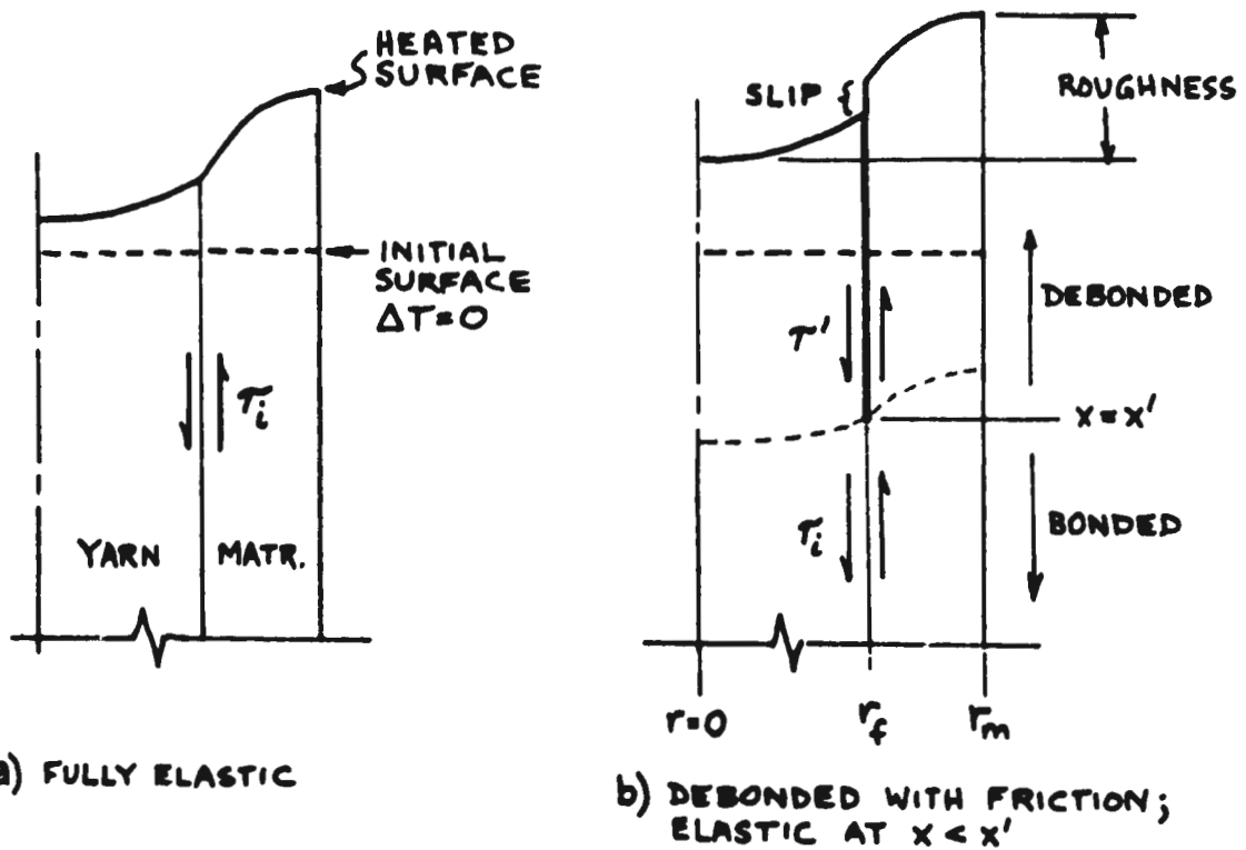
Fig. 3. Schematic of deformations at the free surface.
