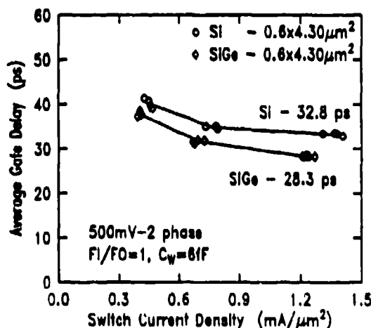
Figure 10 (ref 5) Comparison of ECL delay of Si and SiGe transistors detailed in Table 1.
