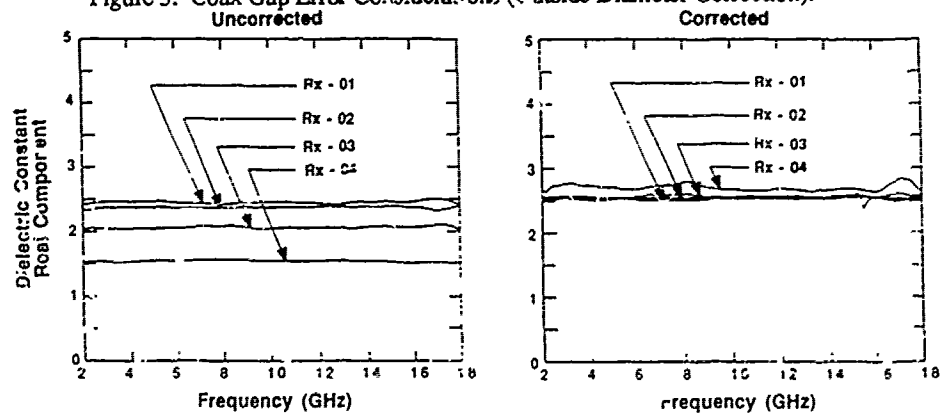
Figure 4. Coax Gap Error Considerations (Inside Diameter Correction).
