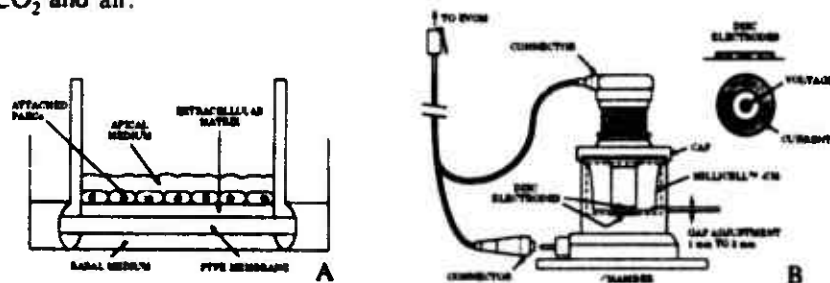
Fig. 1 Millicell CM™ insert (A) showing PTFE Biopore™ membrane, extracellular matrix of type IV collagen, layer of attached PAECs and surround of nutrient medium (apical and basal). Resistance measurement chamber (B) showing EVOM™ connectors, position of the Millicell CM™ insert relative to disc electrodes which face each other from opposite sides of the PAEC tissue sheet. Clearance between the top electrode and PTFE membrane was set at 1-2 mm.
