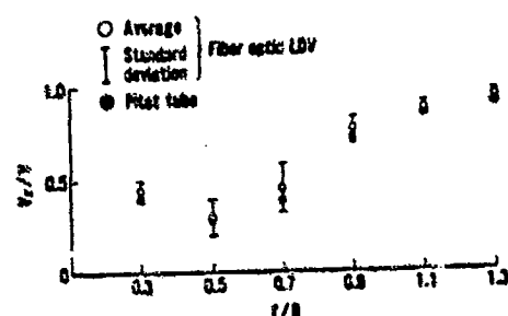
Fig. 4 Comparison of Steady State Velocities Measured by Fiber Optic LDV and 3-Hole Pitot Tube
