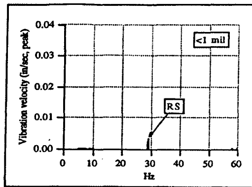
Figure 5. Well-Aligned Vibration Spectrum
