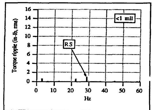
Figure 6. Well-Aligned Torque Ripple Spectrum
