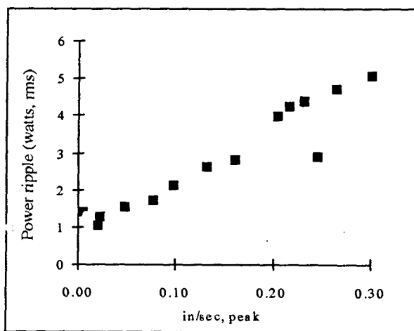
Figure 4. Power Ripple vs. Vibration Amplitude - Running Speed-Related Components for an Unbalanced Rotor
