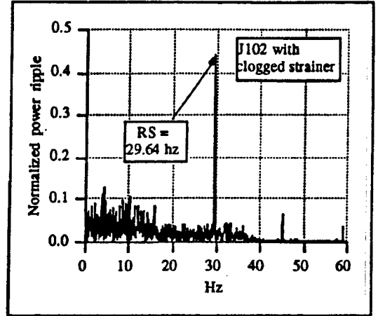
Figure 17. Motor Power Spectrum for Pump with Clogged Suction Strainer
