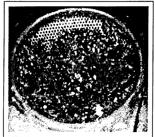
Figure 19. Clogged Suction Strainer
