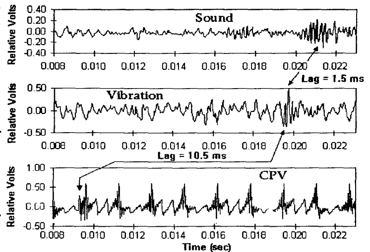
Figure 10 - Sound and vibration pulse comparison
