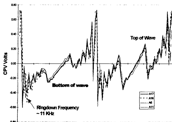
Figure 7 - Comparison of Alternator CPV
