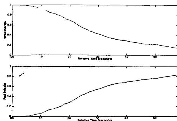
Figure 4: Fault Indicators for F110-GE-129 Turbine
