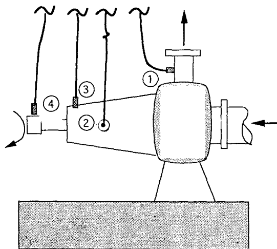
1. Dynamic pressure sensor 2. Accelerometer 3. Bearing defect sensor 4. Speed sensor
