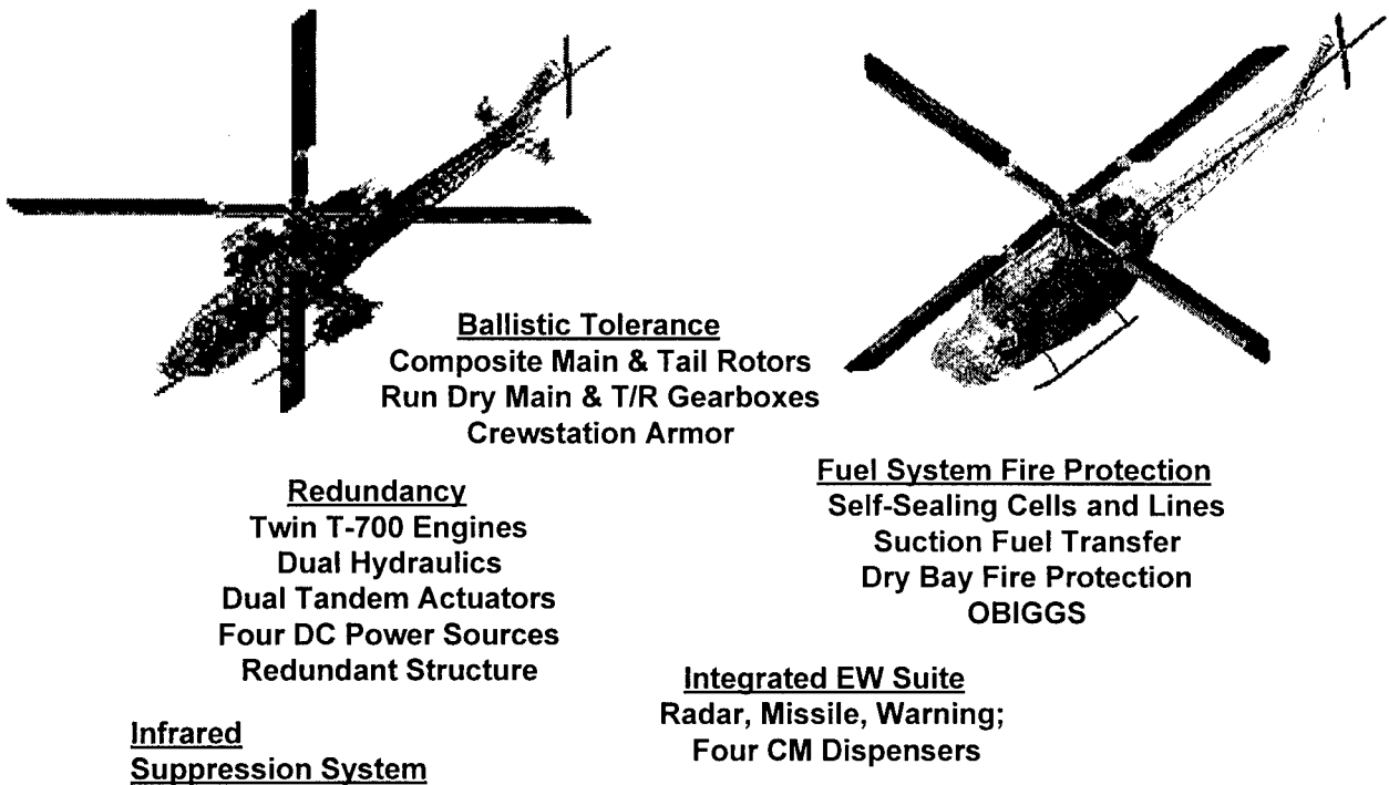
Fig. 17. H-1 survivability features.
