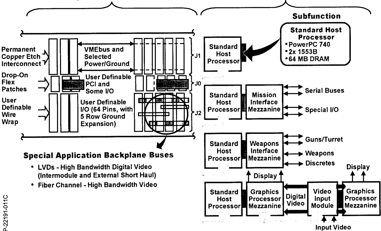
Figure 11. Mission Computer Concepts of Backplane Interconnection and Subfunction Mixing
