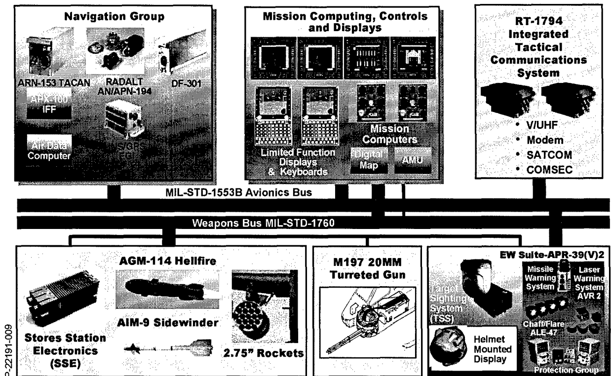
Figure 9. AH-1Z Integrated Avionics System Components and Architecture
