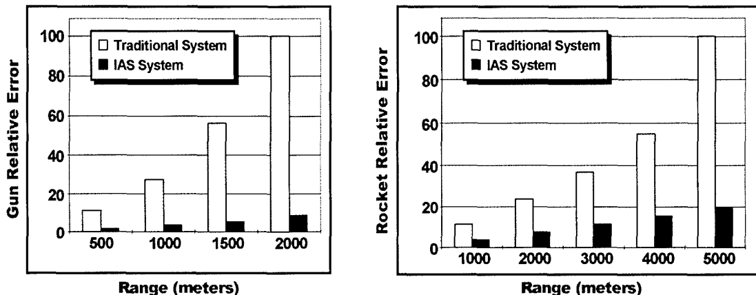
Figure 8. Relative Error Improvements with Integrated Avionics Systems
