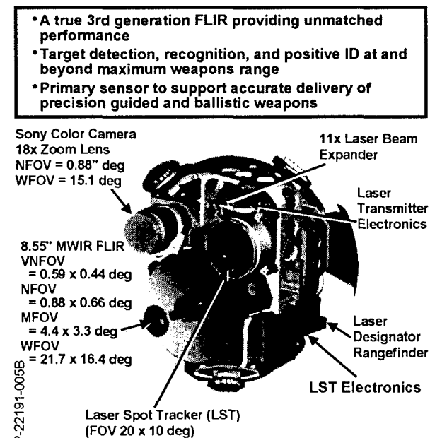
Figure 5. Long-Range Target Sighting System
