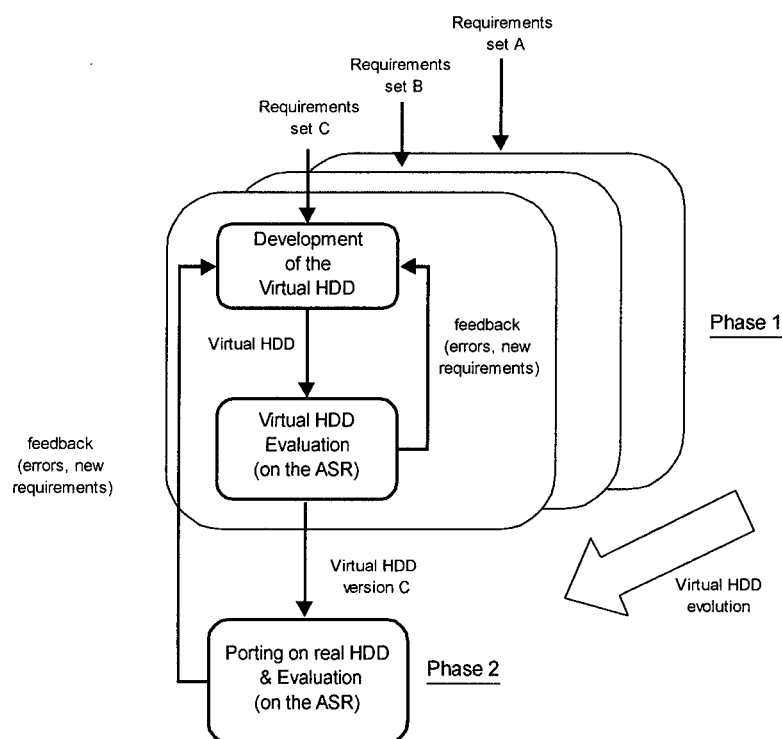
Figure 6: The adopted development process
