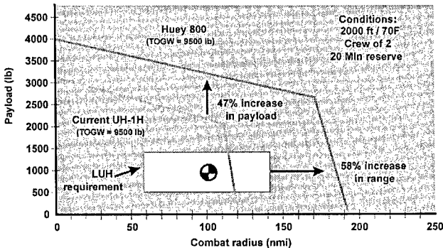
Figure 13. Payload/range comparison.
