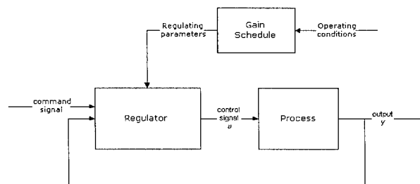
Figure 1. Gain scheduling
