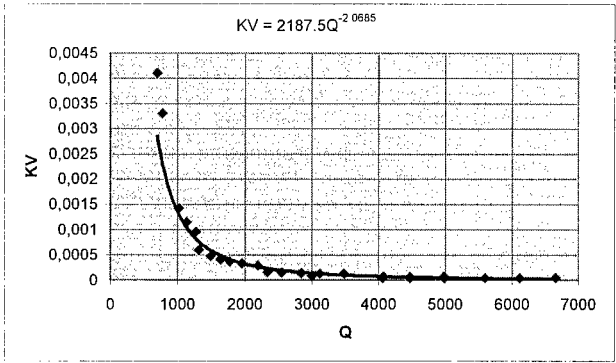
Figure 3-a. Gain vs. dynamic pressure plot and approximate curve fit with its equation for K_v
