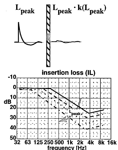
Figure 19 : principle of non linear ear plugs
