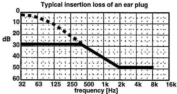
Figure 17 : Typical insertion loss of an ear plug (solid line). The broken line represents the typical IL of a badly fitted plug
