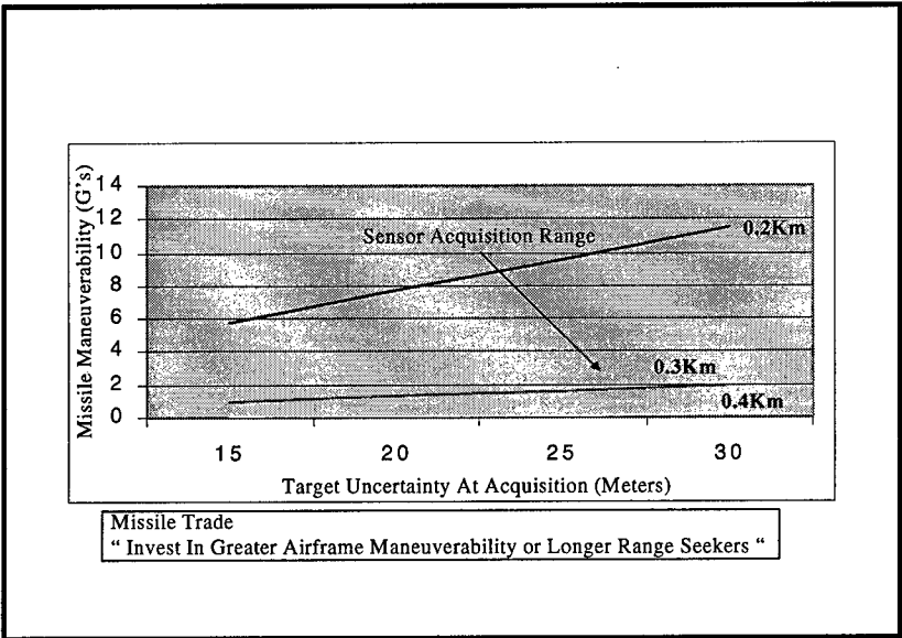
Figure 10 Required Missile Maneuverability
