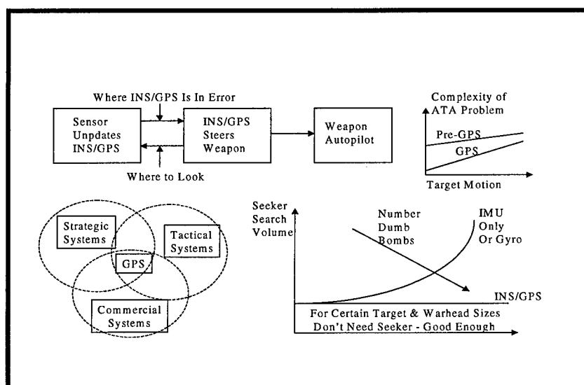
Figure 3 GPS Impact on Seeker Operation
