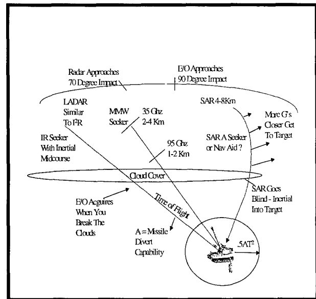
Figure 9 Airframe Seeker Trades
