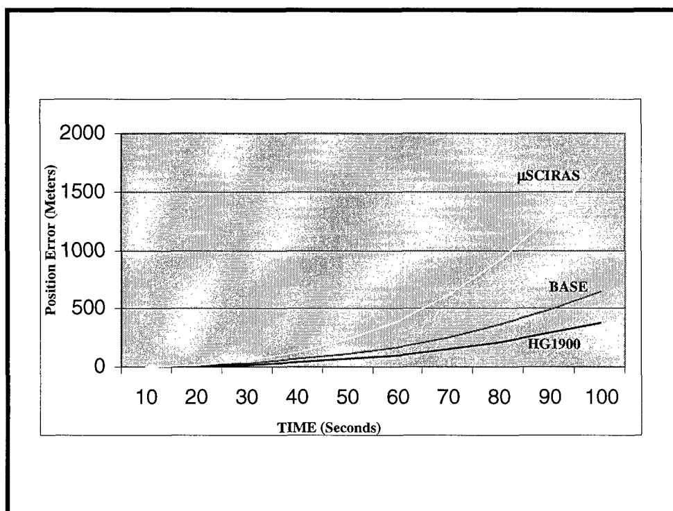
Figure 5. Representative Tactical Grade INS Position Growths
