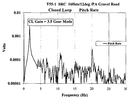
Figure 11 Gravel Road Closed Loop Pitch Rate With gain of 3.5, only gear mode at 2 Hz is unstable. No problem with fuselage bending mode.
