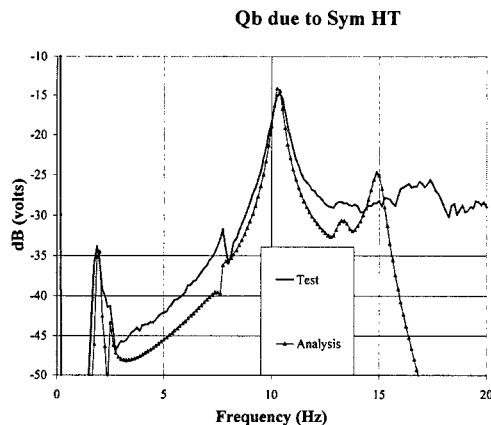
Figure 5a Pitch Rate Structural Transfer Function
