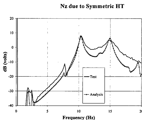
Figure 5b Normal Acceleration Structural Transfer Function
