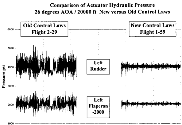
Figure 23 Comparison of Actuator Hydraulic Pressures New versus Old Control Laws for 26 degree AOA
