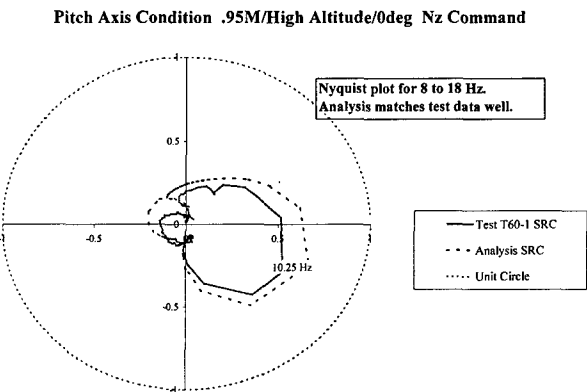
Figure 15 Nyquist Plot for Nz Command
