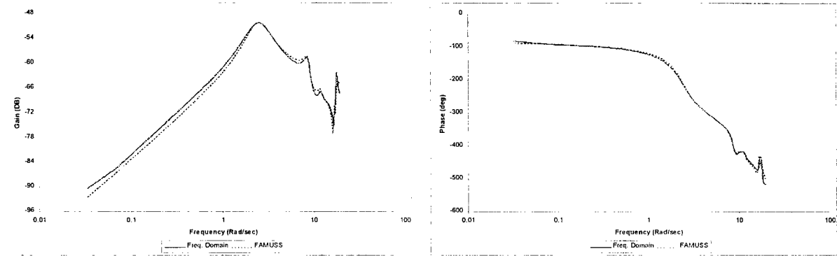
Figure 4: Application of the FAMUSS process to compute CG Acceleration Due to Gust Excitation.
