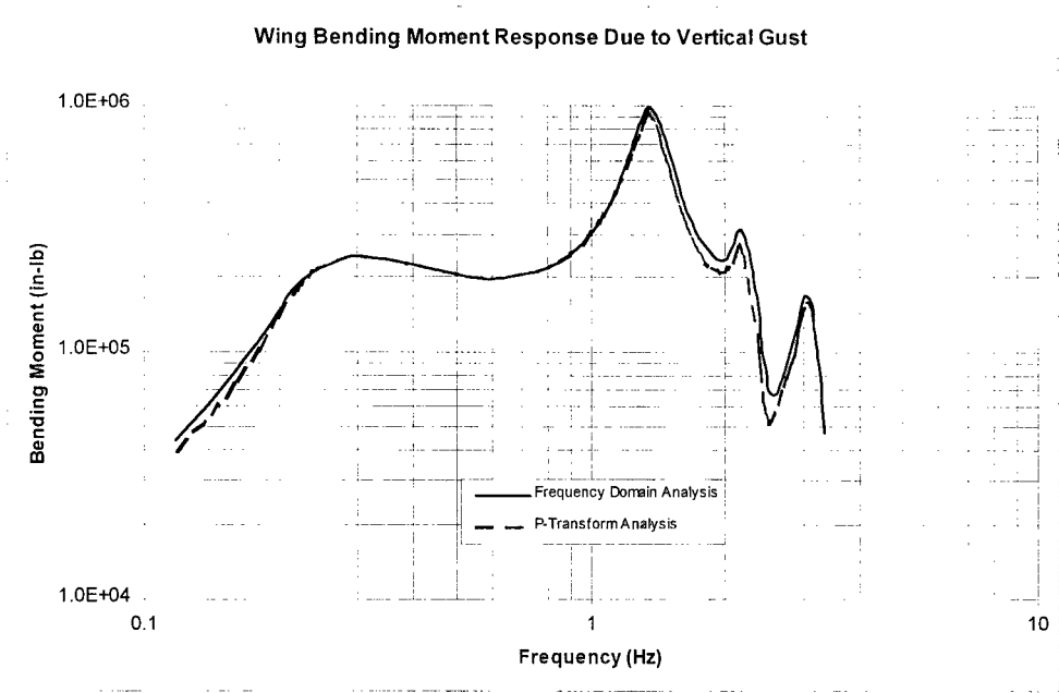
Figure 2: Accuracy of the P-Transform Method for Computing Wing Bending Moments Due to Vertical Gust.
