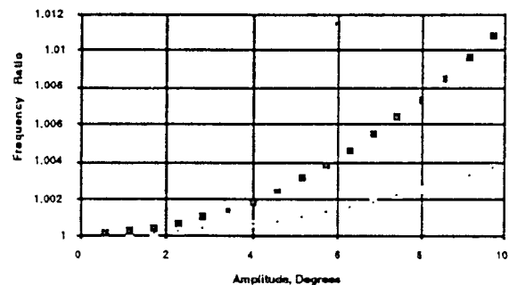
Figure 3. Instability Region for Frequency Ratios near 1
