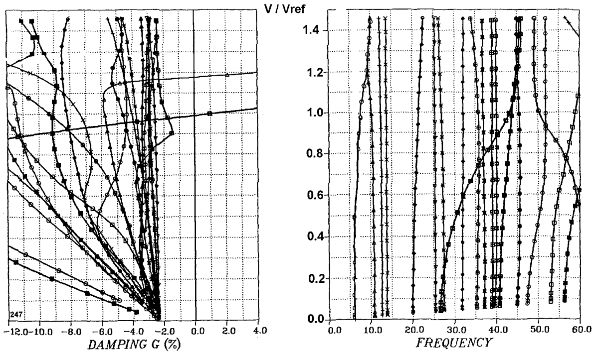
Figure 13: : Damping and Frequency versus Flutterspeed, Mach=1.2, Symmetric, sea level, open loop
