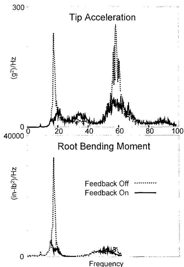
Figure 10. Power Spectral Densities of Buffeting During Feedback Off and On Conditions, Blended Buffeting Alleviation System, Starboard Vertical Tail, 1/6-scale F/A-18 (SIDEKIC) Model
