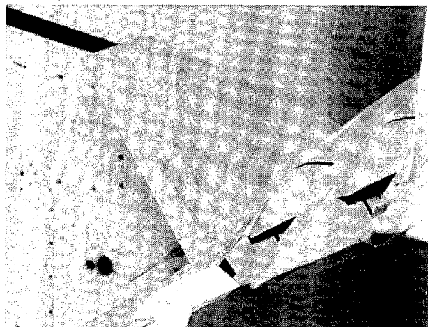
Figure 12. Details of the Flexible Starboard Vertical Tail, 0.135 Scale F-22 Model Mounted in the TDT
