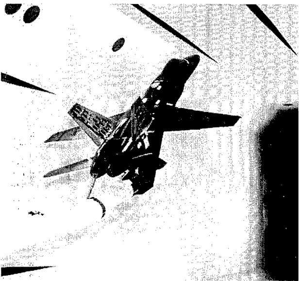
Figure 6. 1/6-scale F/A-18 SIDEKIC Model Mounted in the TDT
