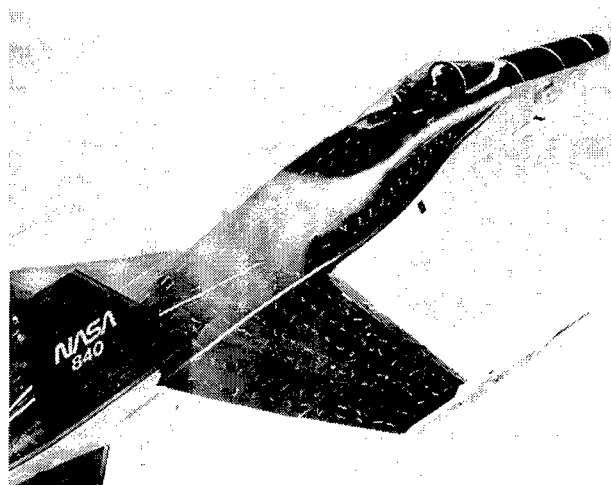
Figure 1. Flow Visualization of Vortex from the LEX Bursting ahead of the Vertical Tail (Photograph Courtesy of the NASA Dryden Flight Research Center)
