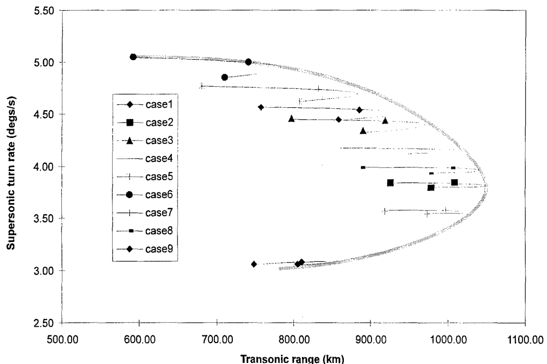
Figure 5. PARETO boundary
