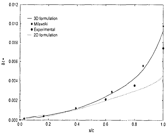
Fig. 11. Chordwise distribution of \delta 1^* at Re = 2.1 \cdot 10^6 , \alpha = 6.3^\circ , 2y/b = 0.5 .
