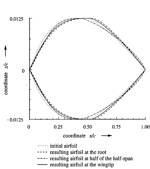
Figure 31: Normalized airfoils of the initial and resulting SCT wing of an optimization at Mach number M_\infty = 2.0 .
