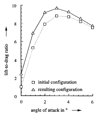
Figure 34: Lift-to-drag ratios of the initial and resulting SCT wing/body configuration resulting from an optimization at Mach number M_\infty = 2.0 and angle of attack \alpha = 3^\circ .
