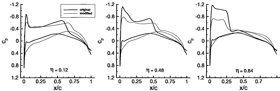
Fig. 16 - Pressure coefficient distributions on the original and optimized (twisted) wings
