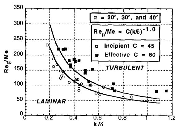
(a) Roughness transition correlation. From Berry et al., 1999.
