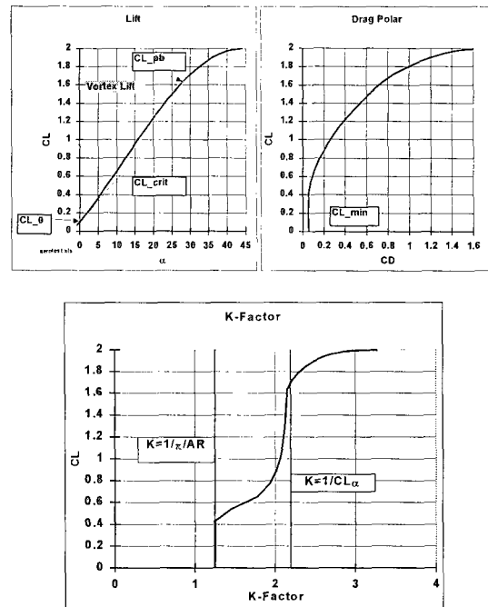
Figure 8: Elements of Lift and Drag Build-up of the clean A/C
