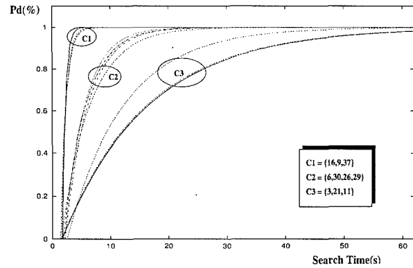
Figure 5: Cumulative distribution functions to the search times for the target scenes
