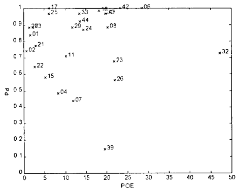
Figure 3. Pd = f(POE)
