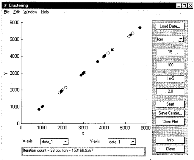
Fig. 11 Clustering results using 15 clusters
