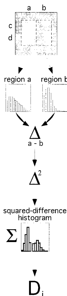
Figure 3. Initial processing steps of the general channel energy model applied to the segregation task of Experiment 1. For each channel-energy "image" a histogram is computed for regions a and b . The histograms are differenced, squared and summed to obtain a measure, D_i , of the histogram difference for each channel.
