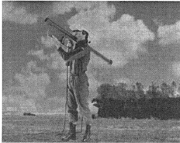
Figure 4. - The HMD based Stinger Trainer concept demonstrator as built by TNO in 1992 (background image is image as seen in the HMD)
