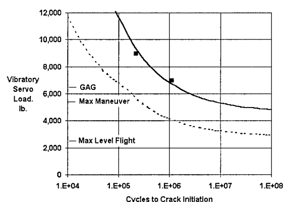
Figure 5. Crack Re-Initiation on Servo Beam Rail
